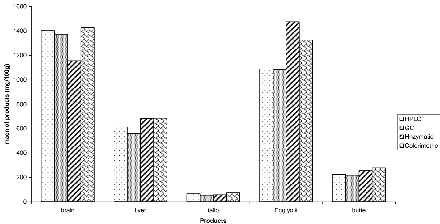
Cholesterol content (mg/100g) in som different food animal sources products determined by HPLC, GC, Enzymatic qnd Colorimetric methods
